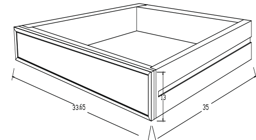
DETAIL DRAWER
