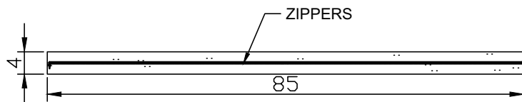
BACK VIEW
